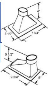
Brake Cooling Ducts available in 2 sizes
